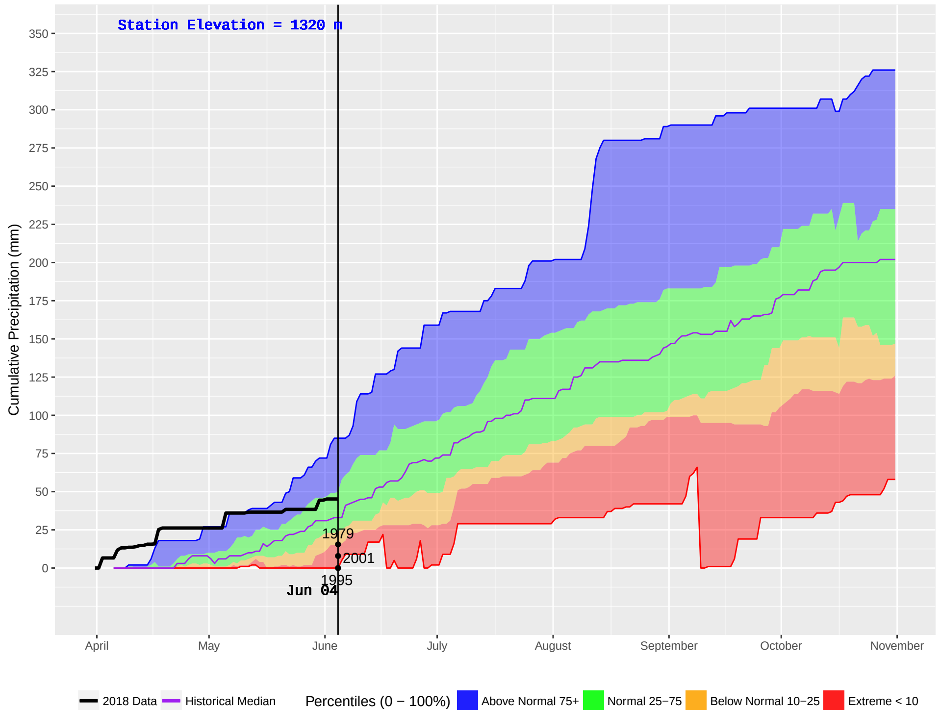
FRENCH BAR (306) : Historical (1979–2016) and Current (2018) Noon Cumulative Precipitation
