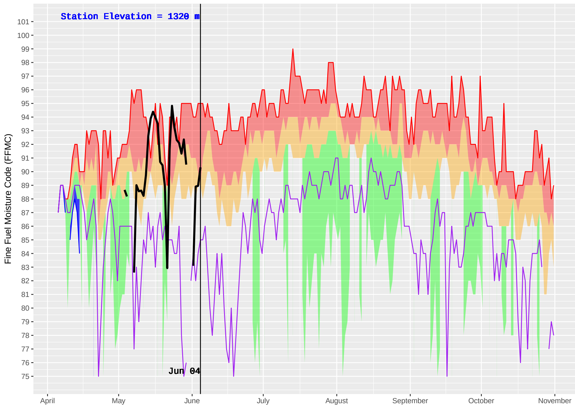
FRENCH BAR (306) : Historical (1979–2016) and Current (2018) Noon Fine Fuel Moisture Code (FFMC)
