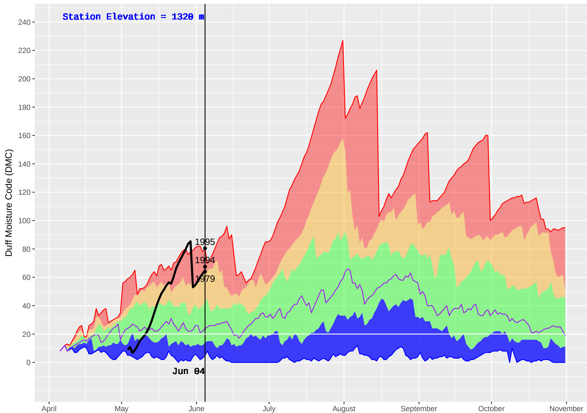
FRENCH BAR (306) : Historical (1979–2016) and Current (2018) Noon Duff Moisture Code (DMC)
