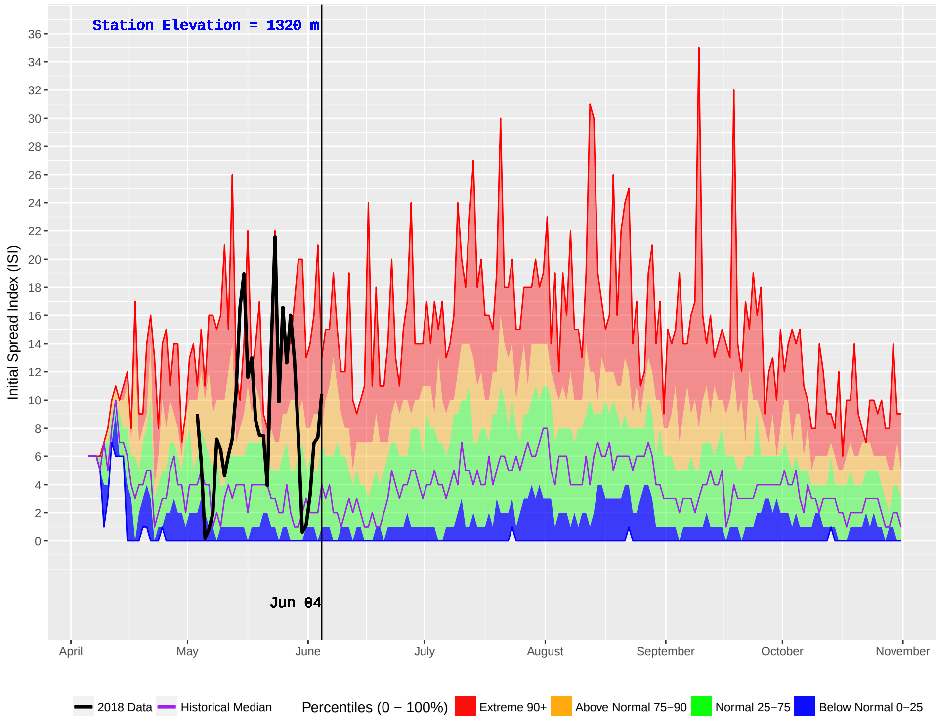
FRENCH BAR (306) : Historical (1979–2016) and Current (2018) Noon Initial Spread Index (ISI)
