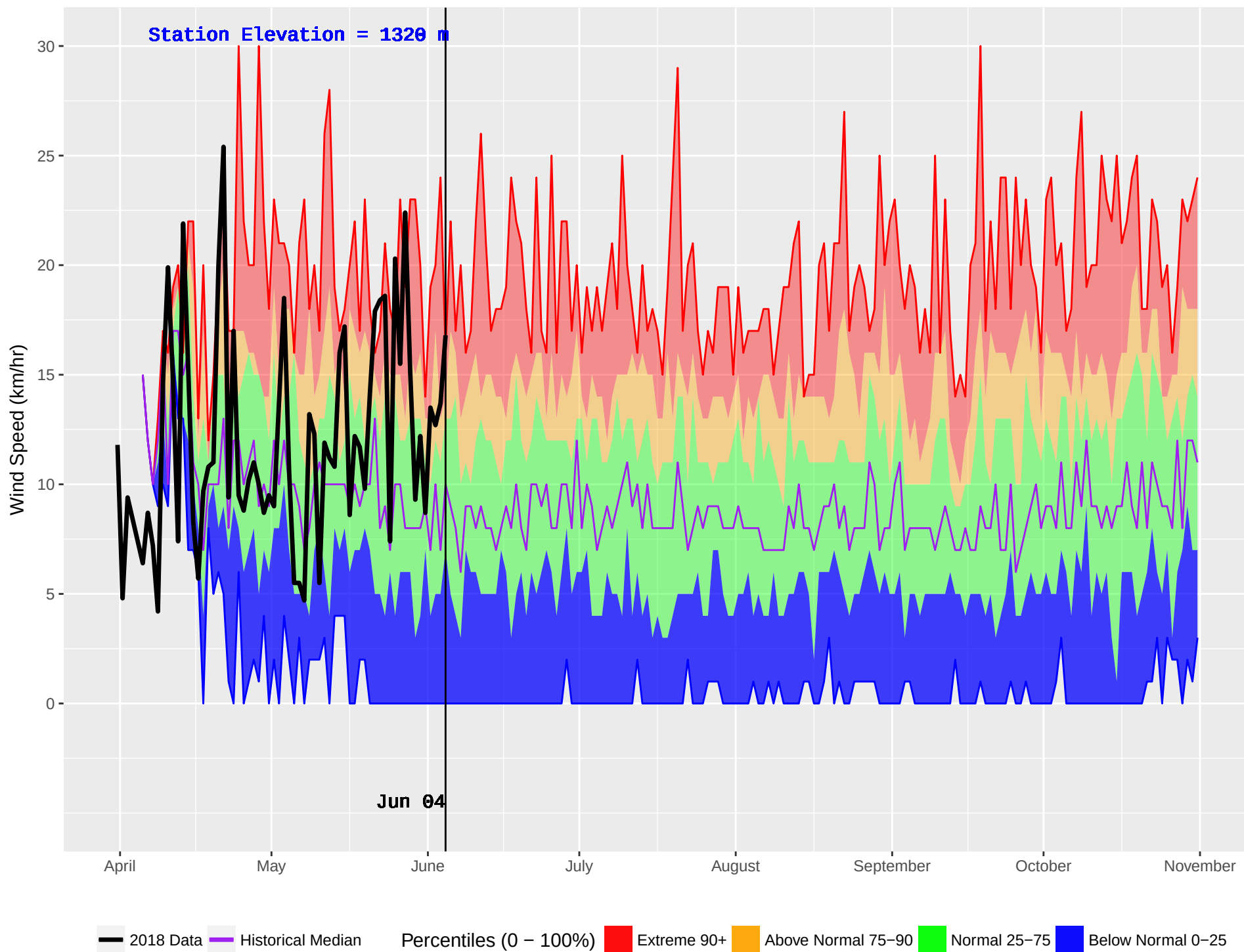
FRENCH BAR (306) : Historical (1979–2016) and Current (2018) Noon Wind Speed
