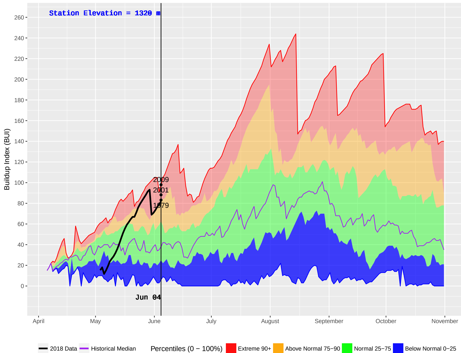
FRENCH BAR (306) : Historical (1979–2016) and Current (2018) Noon Buildup Index (BUI)
