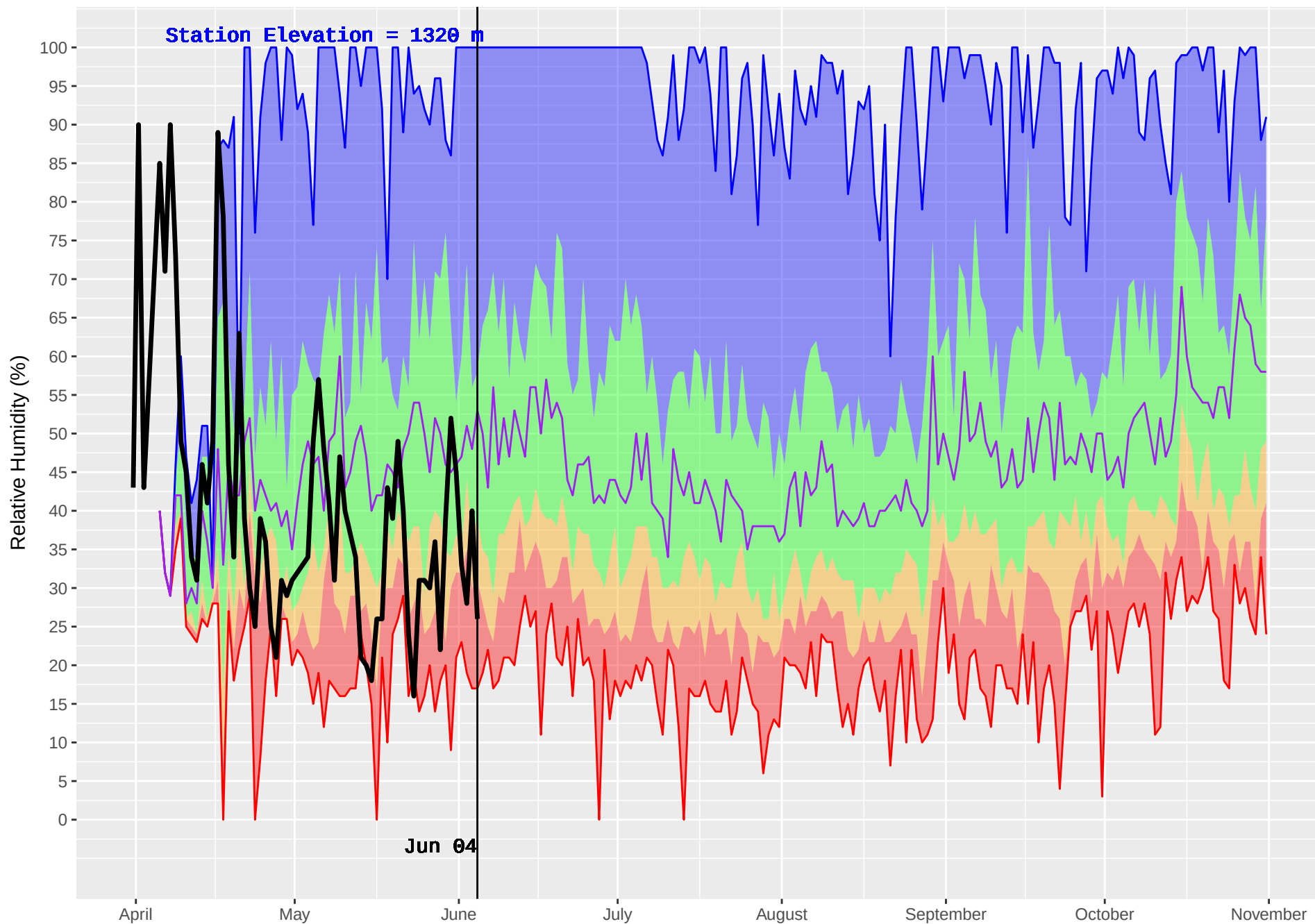
FRENCH BAR (306) : Historical (1979–2016) and Current (2018) Noon Relative Humidity
