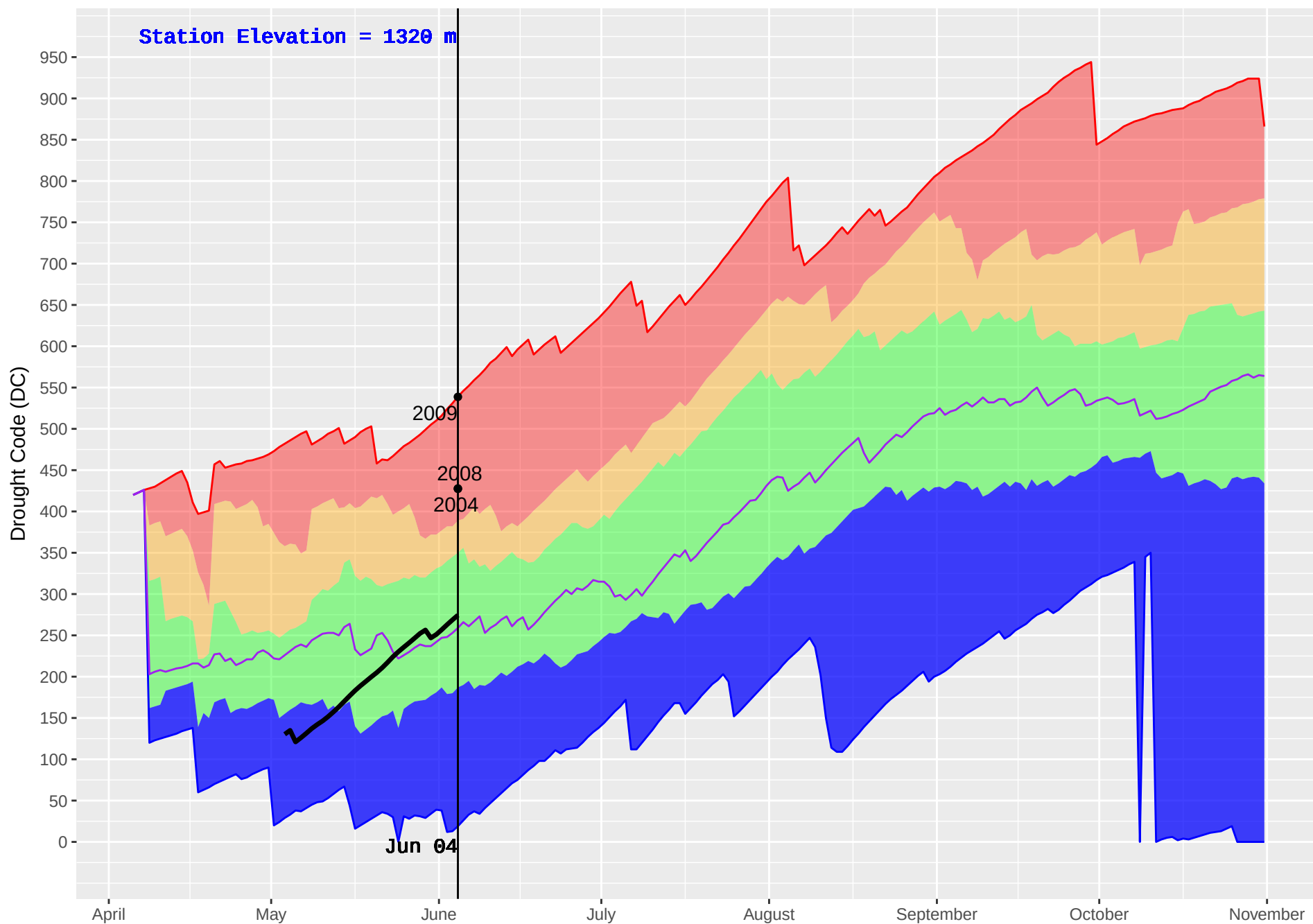
FRENCH BAR (306) : Historical (1979–2016) and Current (2018) Noon Drought Code (DC)
