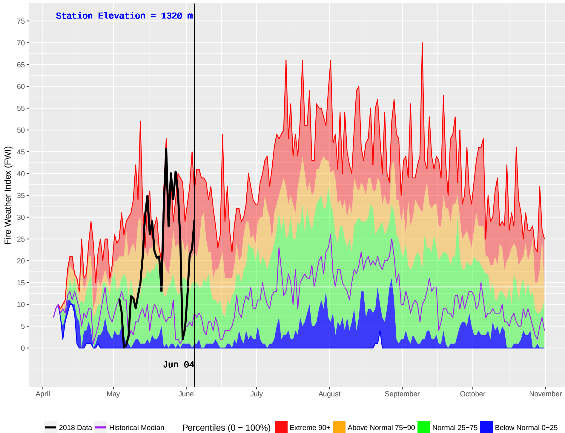
FRENCH BAR (306) : Historical (1979–2016) and Current (2018) Noon Fire Weather Index (FWI)
