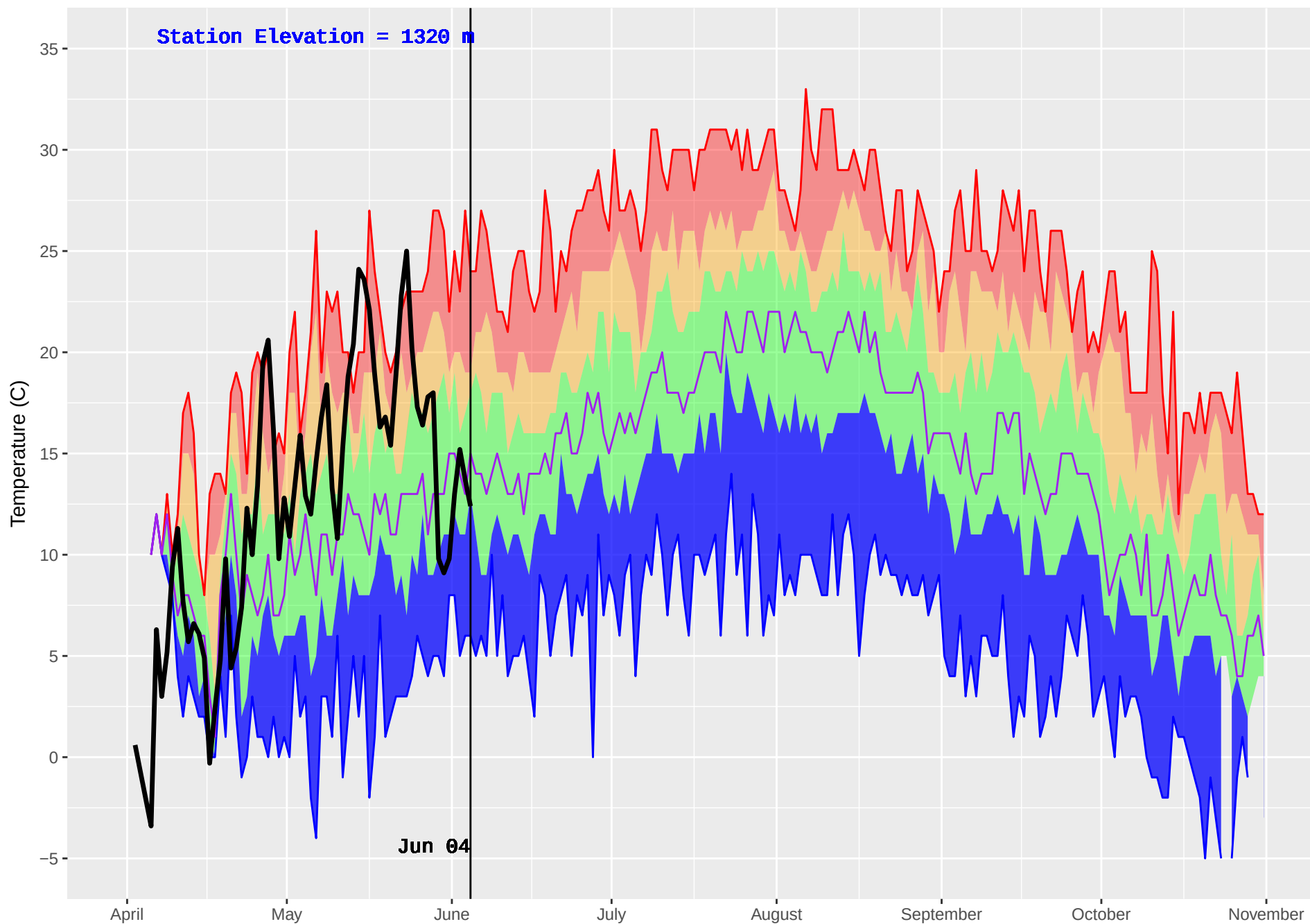
FRENCH BAR (306) : Historical (1979–2016) and Current (2018) Noon Temperature
